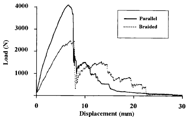
Figure 4. Typical load-displacement curves of a braided doubled gracilis and semitendinosus tendon graft and parallel control.
