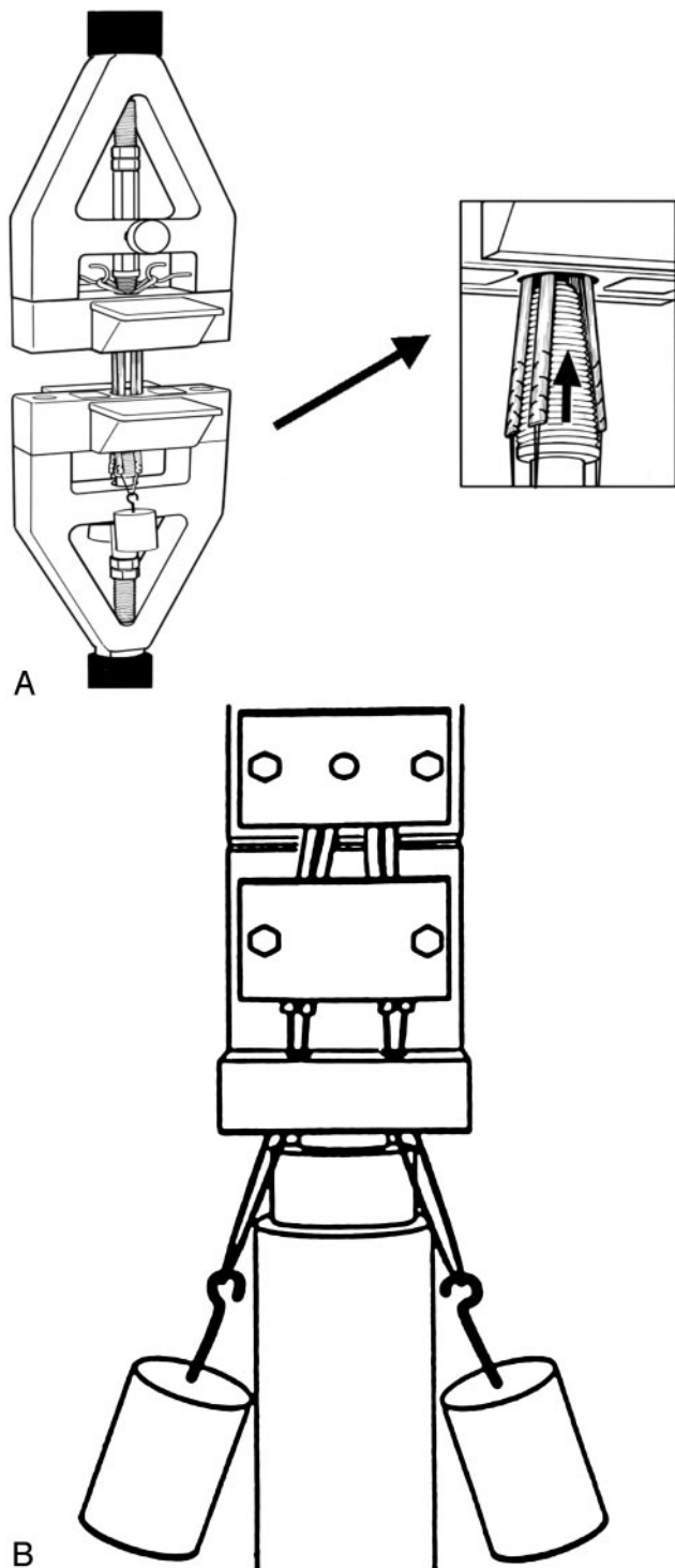
Figure 2. A, at left, the cryogrip system used in the twisting and parallel tendon testing group. This shows four hamstring tendons tested in a parallel orientation and equally tensioned with weights. At right is a close-up illustration of the clamping system, showing fixation of tendons into the bottom clamp. B, the cryogrip system used for the braided and parallel tendon testing group. This shows a parallel doubled gracilis and semitendinosus tendon graft placed in the grips and tensioned with hanging weights.
