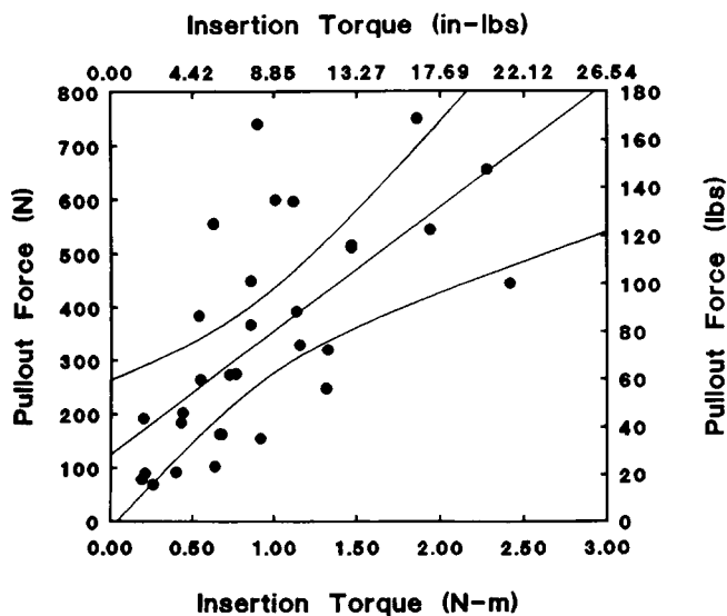
Figure 2. For endoscopically inserted screws of 5.5 and 7 mm diameter and 9 mm inserted outside-in, there is a weak but significant ( r^2 = 0.45 , P < 0.05 ) positive linear correlation between screw insertion torque and measured pullout force.
